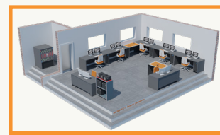
LABORATORY CONFIGURATION
